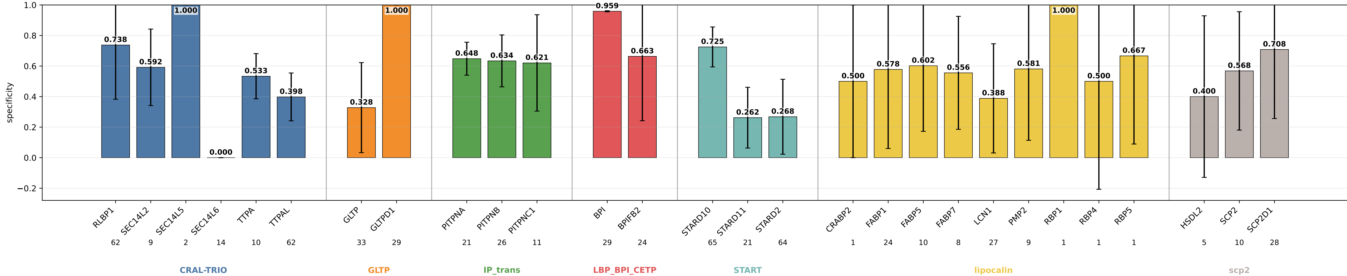
geometric_edge_attention_protgeom8 specificity by subgroup geometric_edge_attention_protgeom8 | class weights | lr=0.0001 | weight_decay=0.01 | final_m=4 | final_dropout=0.1 | hiddim=8 | heads=8 | batch=16 | ep=120 | seeds=0,1,2
