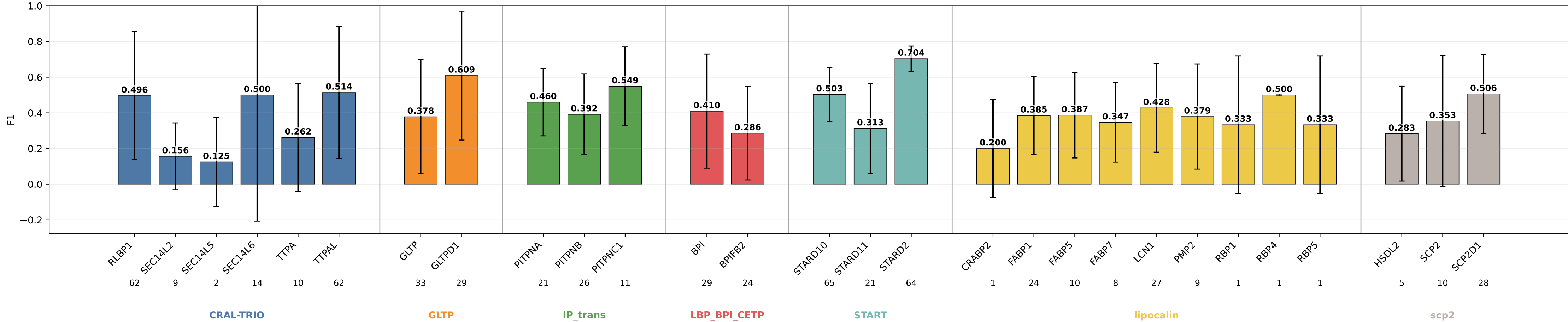
geometric_edge_mlp F1 by subgroup geometric_edge_mlp | class weights | lr=0.0001 | weight_decay=0.01 | final_m=4 | final_dropout=0.1 | hiddim=8 | heads=8 | batch=16 | ep=120 | seeds=0,1,2,3,4
