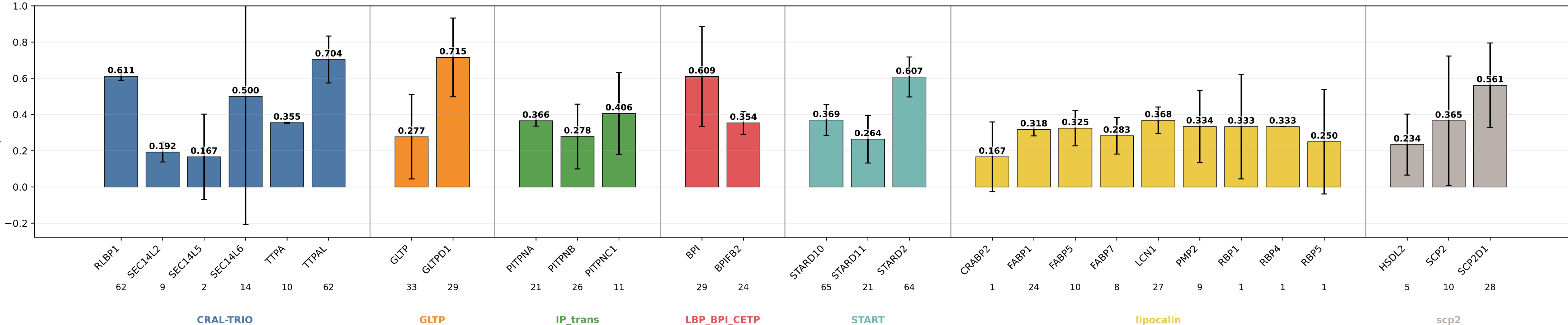
geometric_edge_mlp precision by subgroup geometric_edge_mlp | class weights | lr=0.0001 | weight_decay=0.01 | final_m=4 | final_dropout=0.1 | hiddim=8 | heads=8 | batch=16 | ep=120 | seeds=0,1,2,3,4
