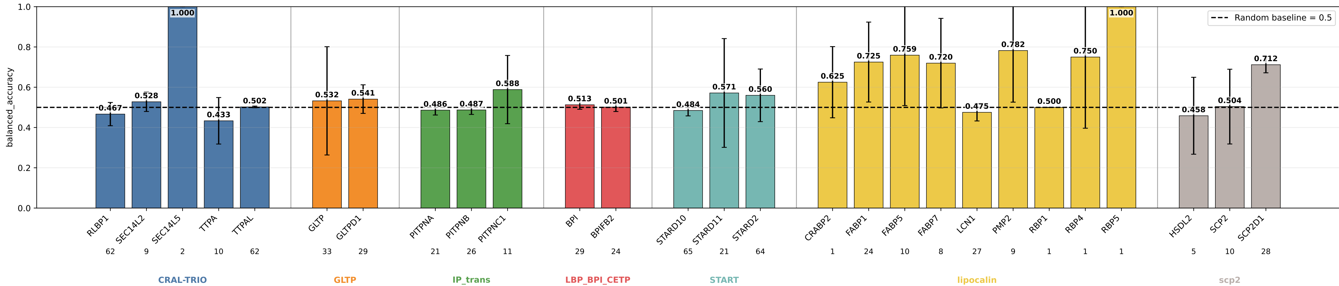
geometric_edge_mlp_add_nwd balanced_accuracy by subgroup geometric_edge_mlp_add_nwd | class weights | lr=0.0001 | weight_decay=1e-05 | final_m=4 | final_dropout=0.1 | hiddim=8 | heads=8 | batch=16 | ep=120 | seeds=0,1,2
