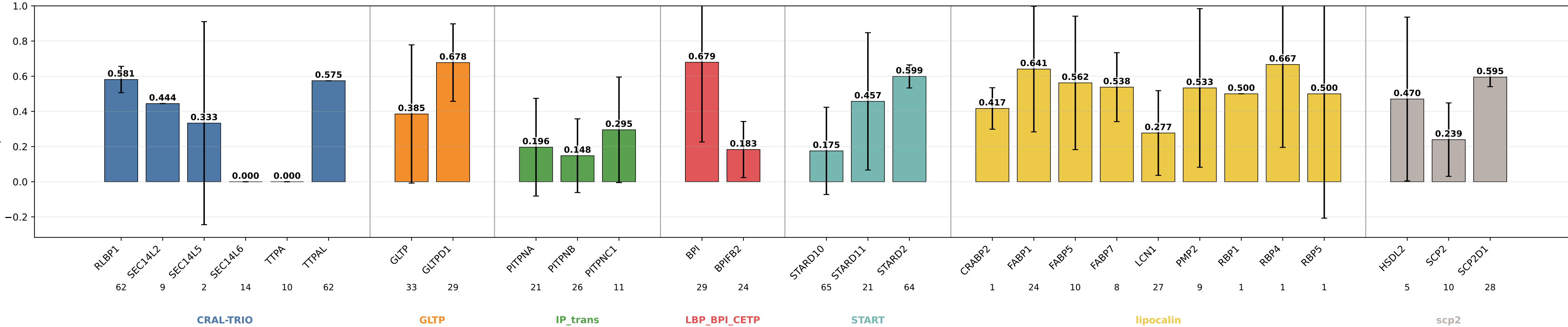
geometric_edge_mlp_add_nwd precision by subgroup geometric_edge_mlp_add_nwd | class weights | lr=0.0001 | weight_decay=1e-05 | final_m=4 | final_dropout=0.1 | hiddim=8 | heads=8 | batch=16 | ep=120 | seeds=0,1,2
