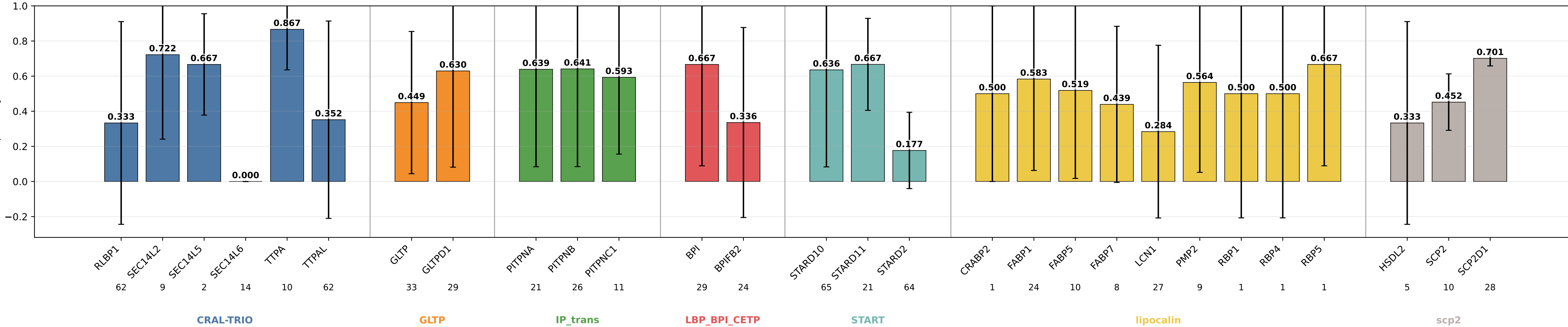
geometric_edge_mlp_add_nwd specificity by subgroup geometric_edge_mlp_add_nwd | class weights | lr=0.0001 | weight_decay=1e-05 | final_m=4 | final_dropout=0.1 | hiddim=8 | heads=8 | batch=16 | ep=120 | seeds=0,1,2
