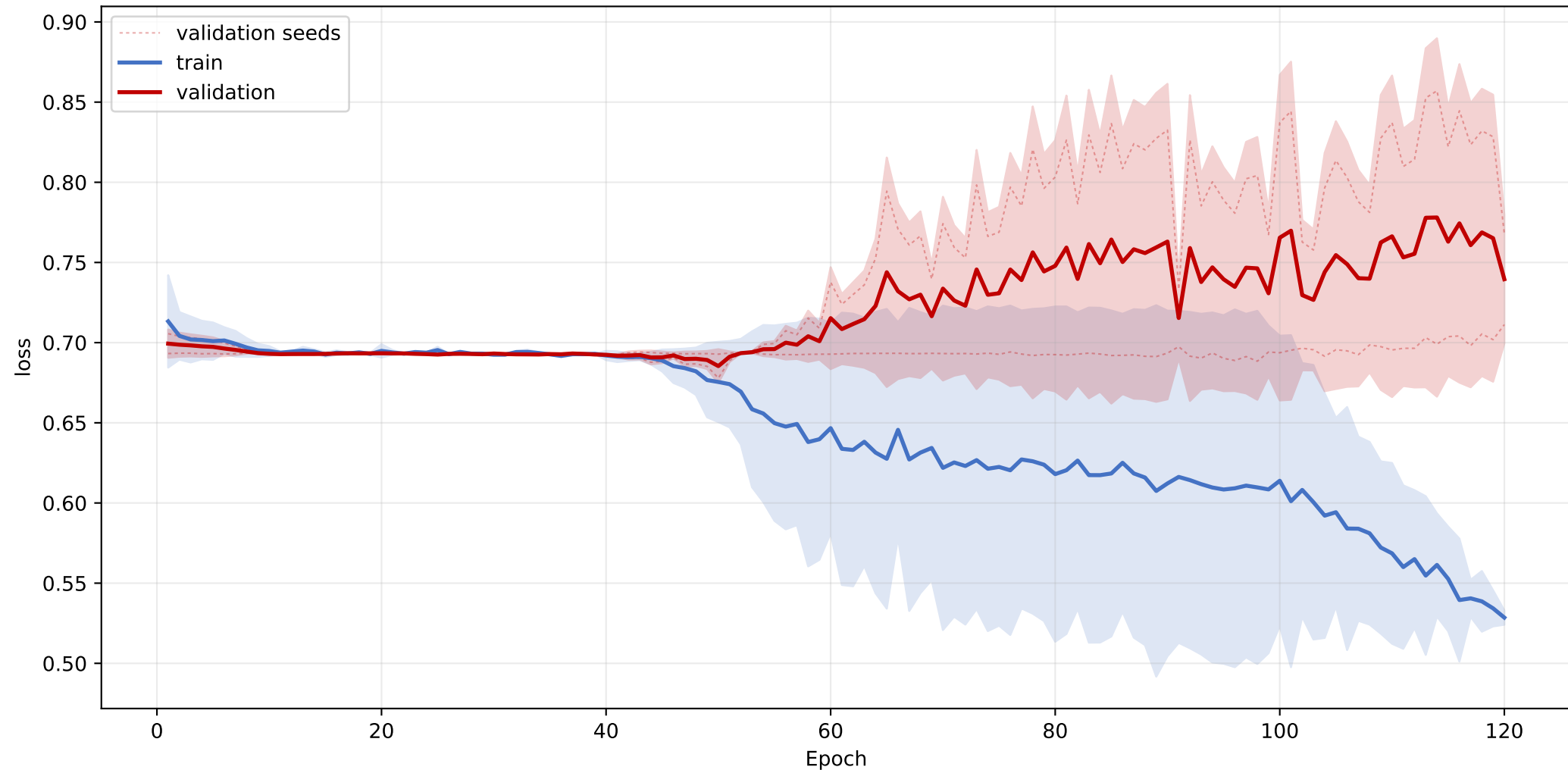
CRAL-TRIO: mean loss learning curve across seeds
