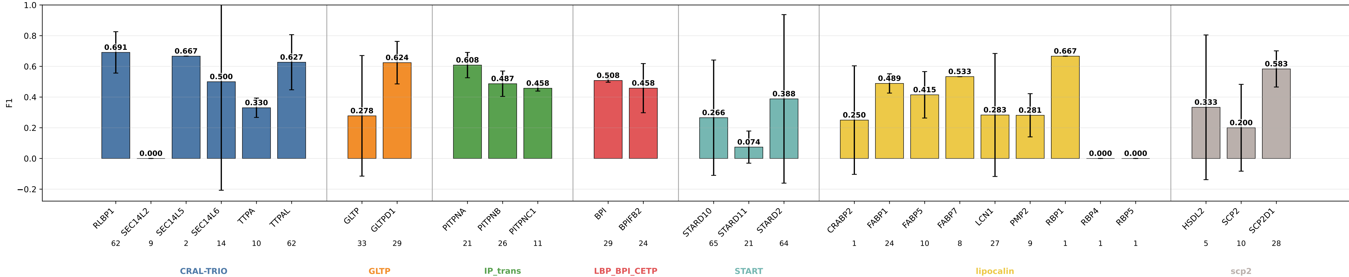
geometric_edge_mlp_nwd F1 by subgroup geometric_edge_mlp_nwd | class weights | lr=0.0001 | weight_decay=1e-05 | final_m=4 | final_dropout=0.1 | hiddim=8 | heads=8 | batch=16 | ep=120 | seeds=0,1
