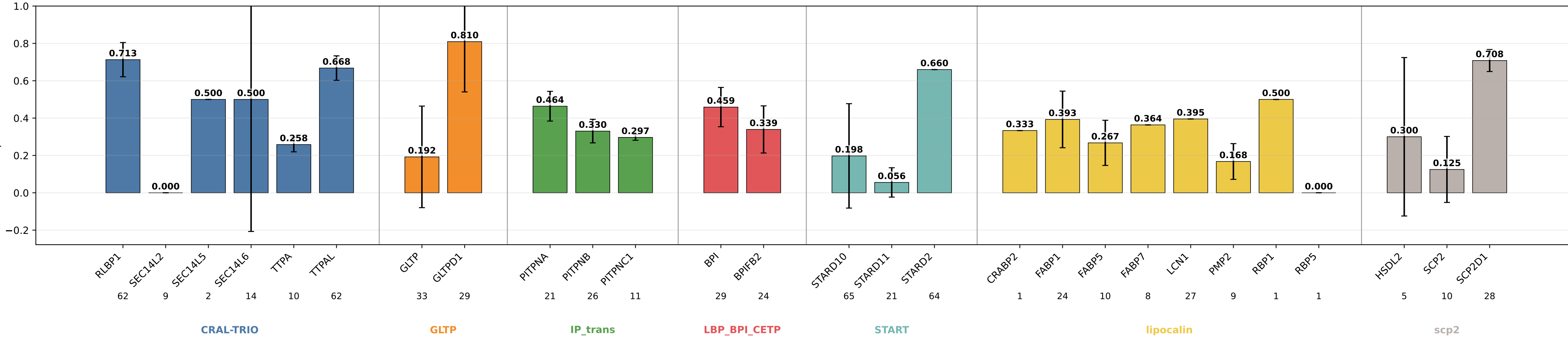
geometric_edge_mlp_nwd precision by subgroup geometric_edge_mlp_nwd | class weights | lr=0.0001 | weight_decay=1e-05 | final_m=4 | final_dropout=0.1 | hiddim=8 | heads=8 | batch=16 | ep=120 | seeds=0,1
