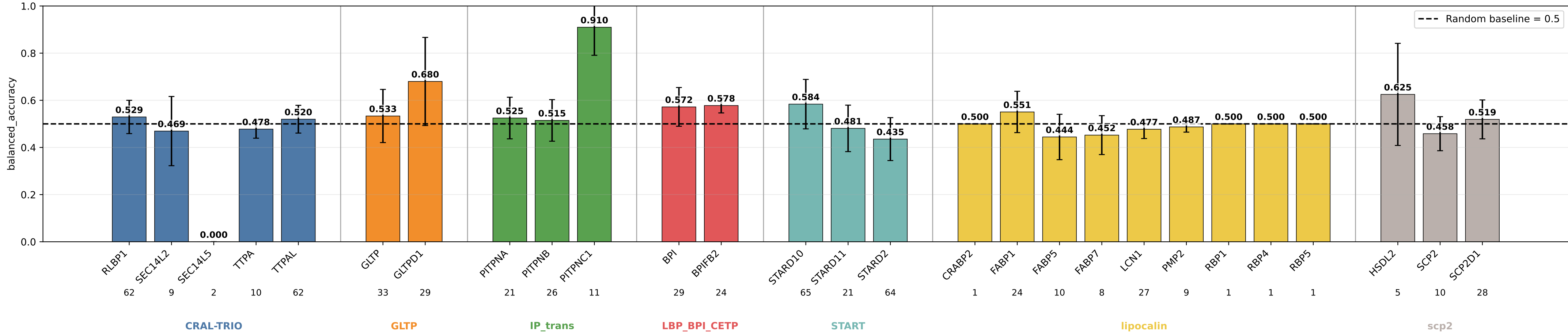
geometric_edge_mlp_nwd_no_lipid_graphs balanced_accuracy by subgroup geometric_edge_mlp_nwd_no_lipid_graphs | class weights | lr=0.0001 | weight_decay=1e-05 | final_m=4 | final_dropout=0.1 | hiddim=8 | heads=8 | batch=16 | ep=120 | seeds=0,1,2
