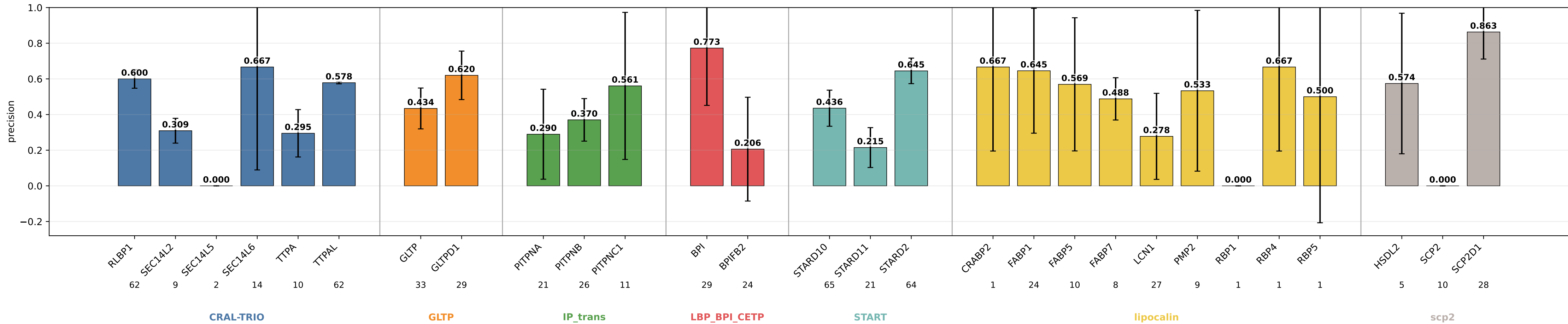
geometric_edge_mlp_nwd_protgeom8_lipprop precision by subgroup geometric_edge_mlp_nwd_protgeom8_lipprop | class weights | lr=0.0001 | weight_decay=0.01 | final_m=4 | final_dropout=0.1 | hiddim=8 | heads=8 | batch=16 | ep=120 | seeds=0,1,2
