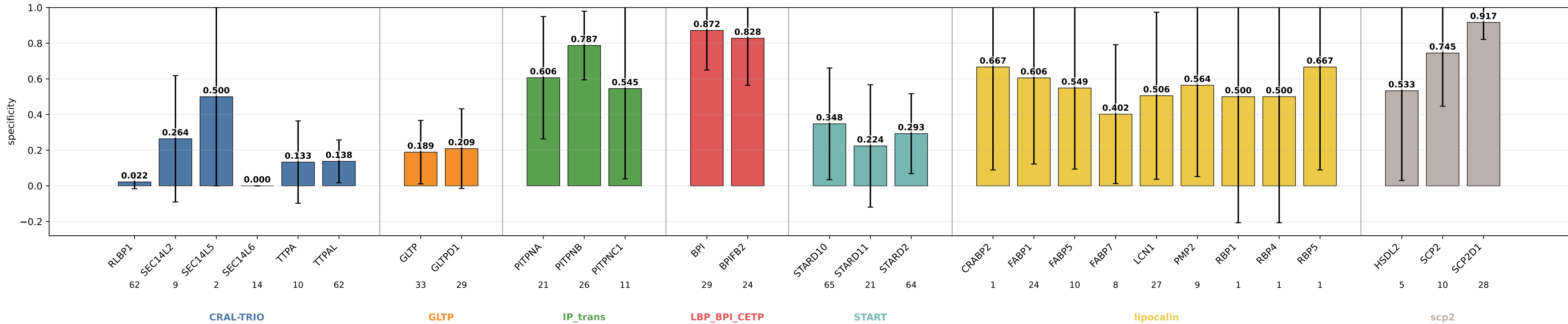
geometric_edge_mlp_nwd_protgeom8_lipprop specificity by subgroup geometric_edge_mlp_nwd_protgeom8_lipprop | class weights | lr=0.0001 | weight_decay=0.01 | final_m=4 | final_dropout=0.1 | hiddim=8 | heads=8 | batch=16 | ep=120 | seeds=0,1,2
