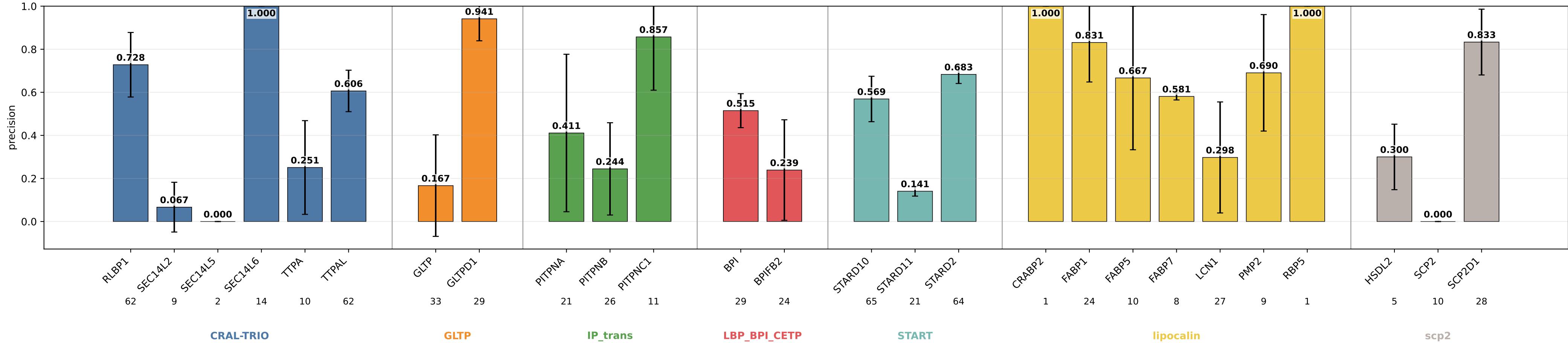
geometric_edge_mlp_protgeom8 precision by subgroup geometric_edge_mlp_protgeom8 | class weights | lr=0.0001 | weight_decay=0.01 | final_m=4 | final_dropout=0.1 | hiddim=8 | heads=8 | batch=16 | ep=120 | seeds=0,1,2
