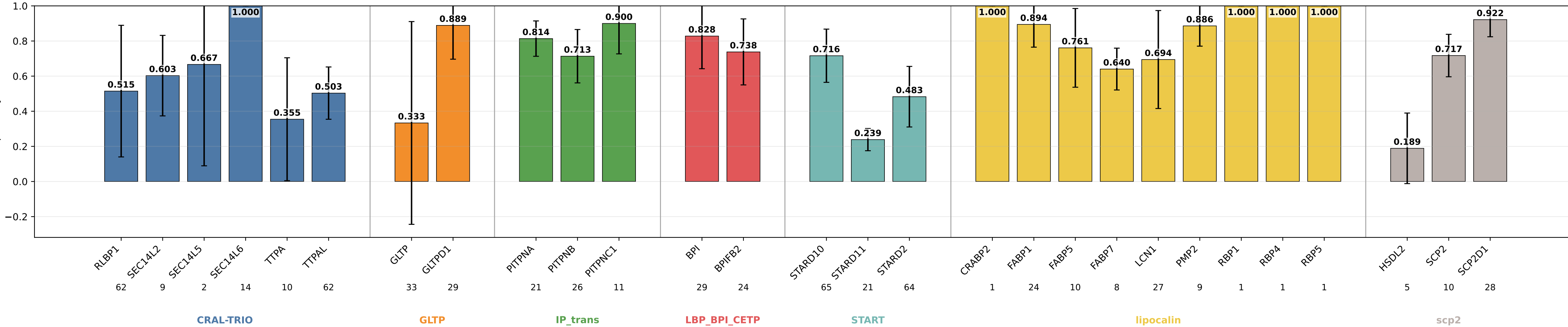
geometric_edge_mlp_protgeom8 specificity by subgroup geometric_edge_mlp_protgeom8 | class weights | lr=0.0001 | weight_decay=0.01 | final_m=4 | final_dropout=0.1 | hiddim=8 | heads=8 | batch=16 | ep=120 | seeds=0,1,2
