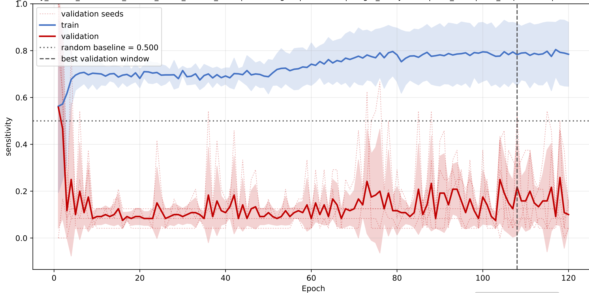
LBP_BPI_CETP: mean sensitivity learning curve across seeds
