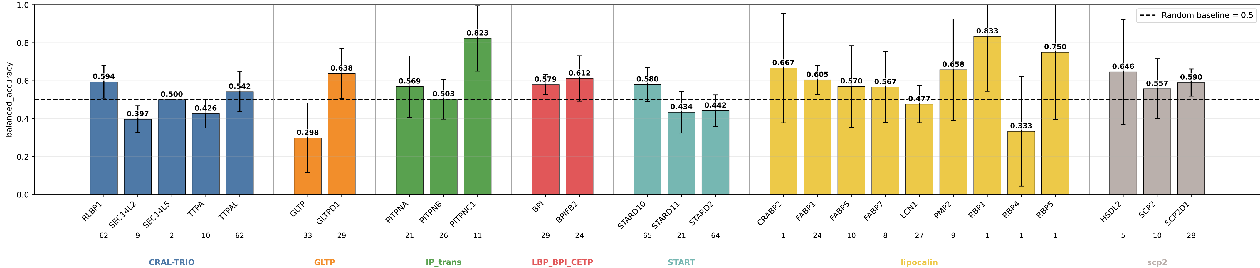
geometric_edge_attention_protgeom_family_neutral_normalized_bilinear_fusion_bilinear_norm balanced_accuracy by subgroup geometric_edge_attention_protgeom_family_neutral_normalized_bilinear_fusion_bilinear_norm | class weights | lr=0.0001 | weight_decay=0.01 | final_m=4 | final_dropout=0.1 | hiddim=8 | heads=8 | batch=16 | ep=120 | seeds=0,1,2,3,4
