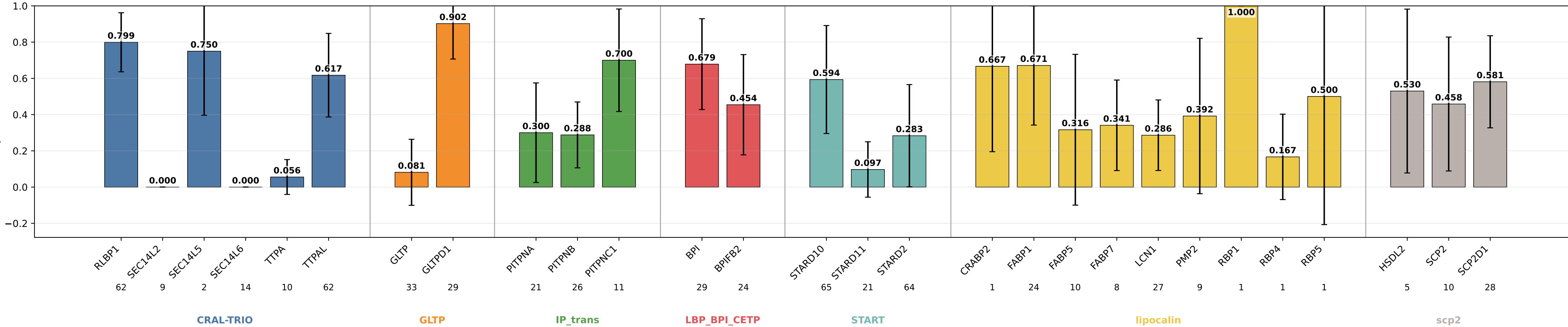
geometric_edge_attention_protgeom_family_neutral_normalized_bilinear_fusion_bilinear_norm precision by subgroup geometric_edge_attention_protgeom_family_neutral_normalized_bilinear_fusion_bilinear_norm | class weights | lr=0.0001 | weight_decay=0.01 | final_m=4 | final_dropout=0.1 | hiddim=8 | heads=8 | batch=16 | ep=120 | seeds=0,1,2,3,4
