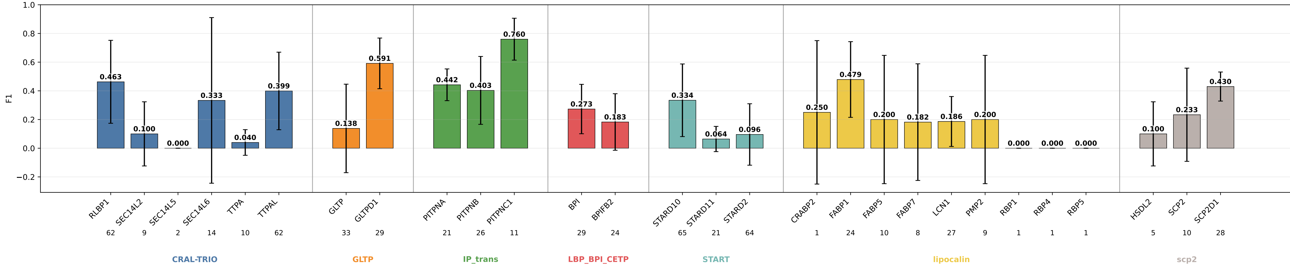
geometric_edge_attention_protgeom_family_neutral_normalized_bilinear_fusion_bilinear_norm_hid16 F1 by subgroup geometric_edge_attention_protgeom_family_neutral_normalized_bilinear_fusion_bilinear_norm_hid16 | class weights | lr=0.0001 | weight_decay=0.01 | final_m=4 | final_dropout=0.1 | hiddim=16 | heads=8 | batch=16 | ep=120 | seeds=0,1,2,3,4
