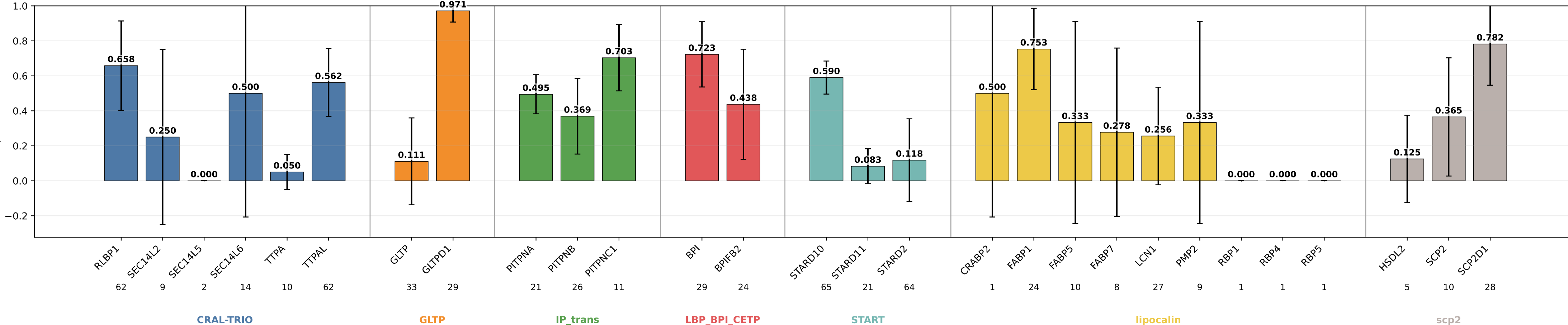
geometric_edge_attention_protgeom_family_neutral_normalized_bilinear_fusion_bilinear_norm_hid16 precision by subgroup geometric_edge_attention_protgeom_family_neutral_normalized_bilinear_fusion_bilinear_norm_hid16 | class weights | lr=0.0001 | weight_decay=0.01 | final_m=4 | final_dropout=0.1 | hiddim=16 | heads=8 | batch=16 | ep=120 | seeds=0,1,2,3,4
