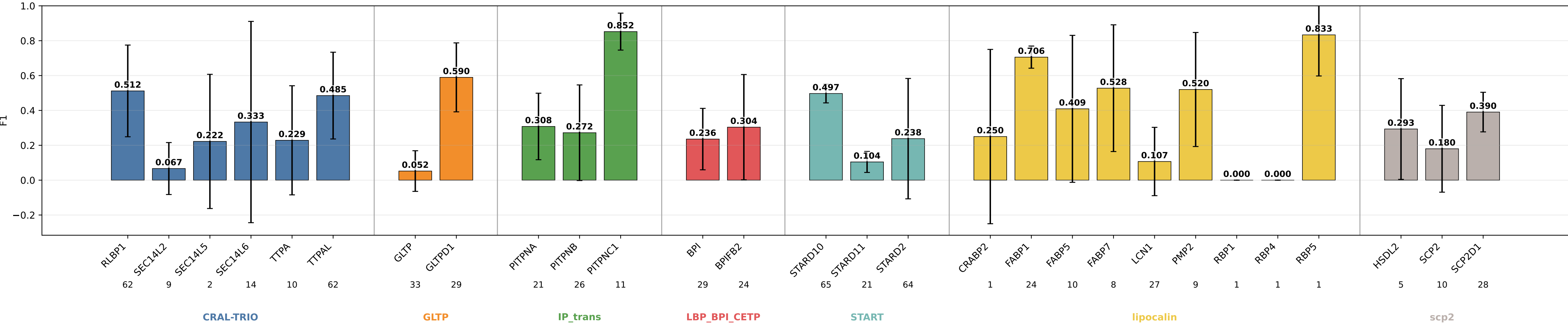
geometric_edge_attention_protgeom_family_neutral_normalized_bilinear_fusion_bilinear_norm_rim_ev28 F1 by subgroup geometric_edge_attention_protgeom_family_neutral_normalized_bilinear_fusion_bilinear_norm_rim_ev28 | class weights | lr=0.0001 | weight_decay=0.01 | final_m=4 | final_dropout=0.1 | hiddim=8 | heads=8 | batch=16 | ep=120 | seeds=0,1,2,3,4
