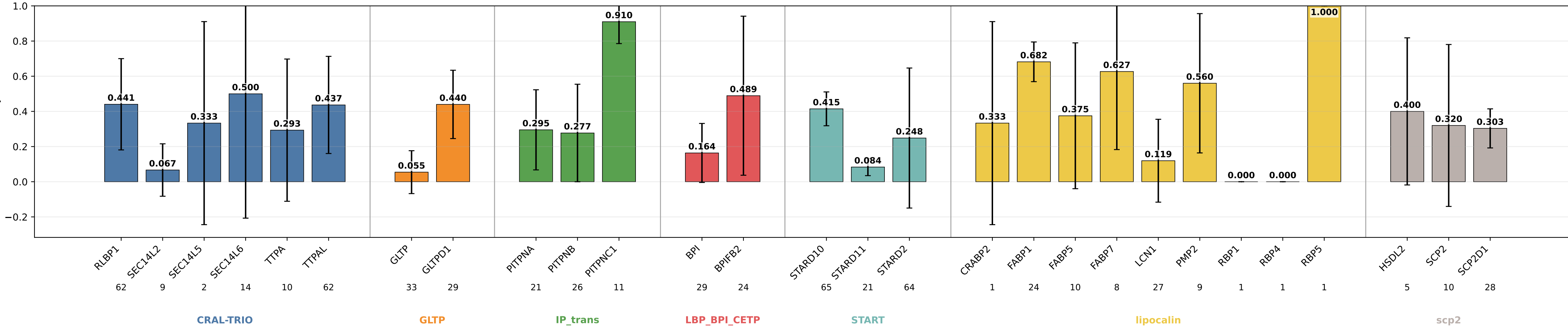
geometric_edge_attention_protgeom_family_neutral_normalized_bilinear_fusion_bilinear_norm_rim_ev28 sensitivity by subgroup geometric_edge_attention_protgeom_family_neutral_normalized_bilinear_fusion_bilinear_norm_rim_ev28 | class weights | lr=0.0001 | weight_decay=0.01 | final_m=4 | final_dropout=0.1 | hiddim=8 | heads=8 | batch=16 | ep=120 | seeds=0,1,2,3,4
