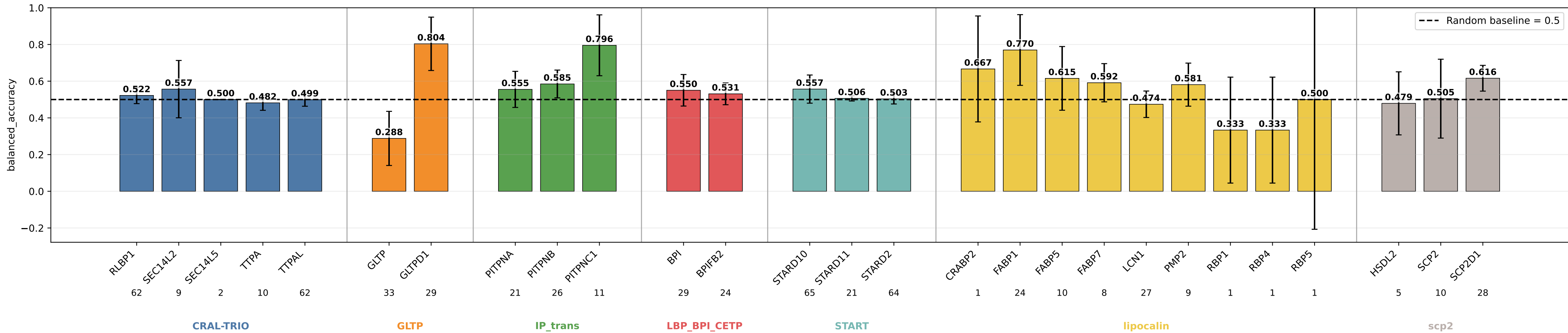
geometric_edge_mlp_protgeom8_normalized_rankprot balanced_accuracy by subgroup geometric_edge_mlp_protgeom8_normalized_rankprot | class weights | lr=0.0001 | weight_decay=0.01 | final_m=4 | final_dropout=0.1 | hiddim=8 | heads=8 | batch=32 | ep=120 | seeds=0,1,2,3,4
