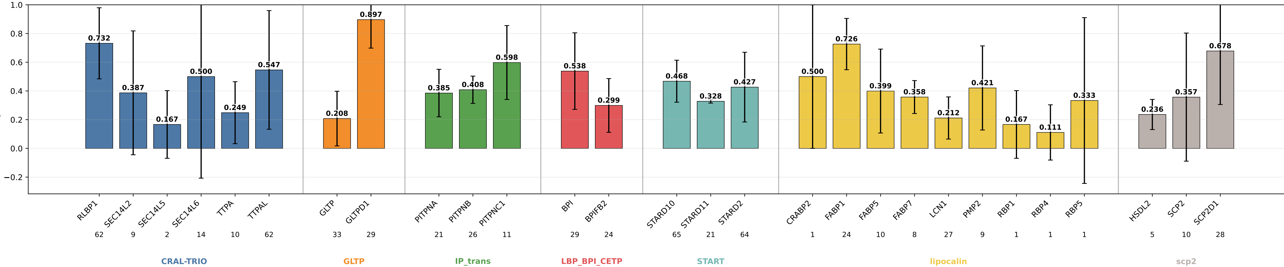
geometric_edge_mlp_protgeom8_normalized_rankprot precision by subgroup geometric_edge_mlp_protgeom8_normalized_rankprot | class weights | lr=0.0001 | weight_decay=0.01 | final_m=4 | final_dropout=0.1 | hiddim=8 | heads=8 | batch=32 | ep=120 | seeds=0,1,2,3,4
