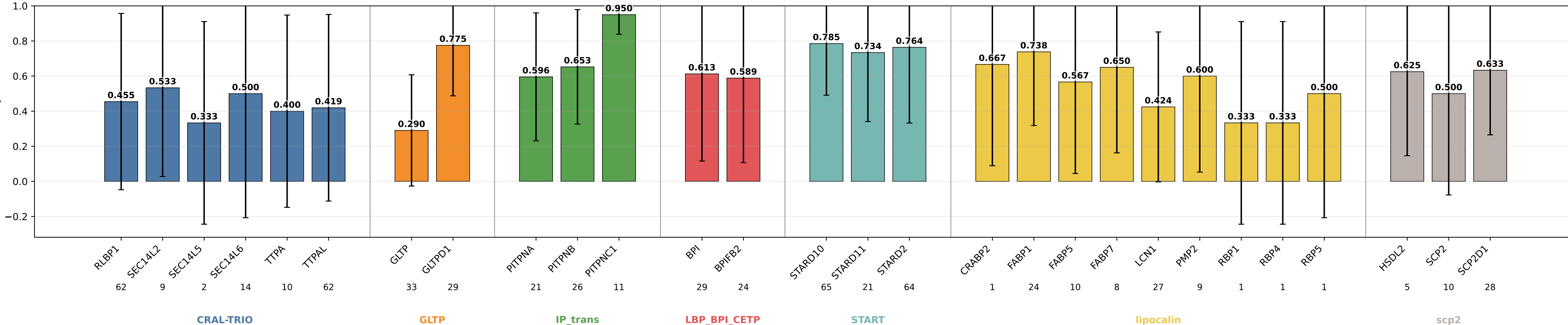
geometric_edge_mlp_protgeom8_normalized_rankprot sensitivity by subgroup geometric_edge_mlp_protgeom8_normalized_rankprot | class weights | lr=0.0001 | weight_decay=0.01 | final_m=4 | final_dropout=0.1 | hiddim=8 | heads=8 | batch=32 | ep=120 | seeds=0,1,2,3,4
