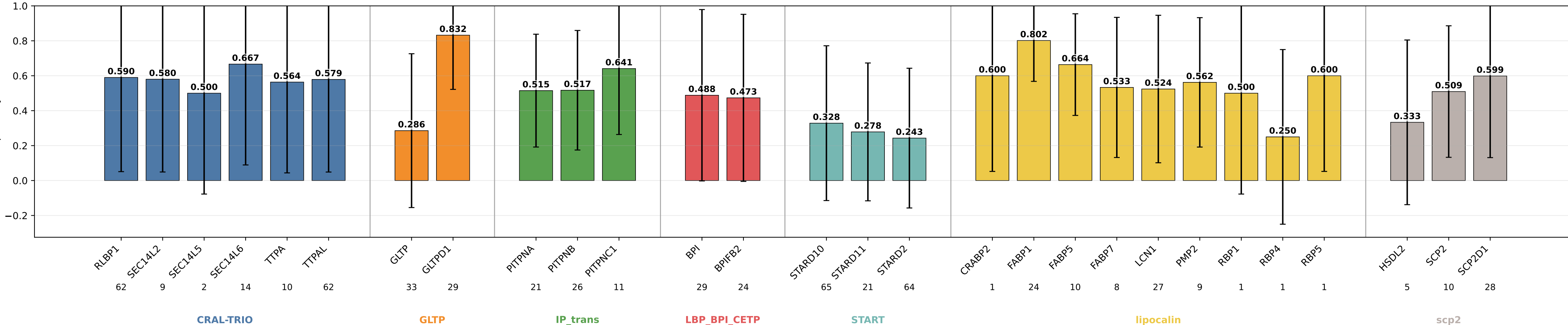
geometric_edge_mlp_protgeom8_normalized_rankprot specificity by subgroup geometric_edge_mlp_protgeom8_normalized_rankprot | class weights | lr=0.0001 | weight_decay=0.01 | final_m=4 | final_dropout=0.1 | hiddim=8 | heads=8 | batch=32 | ep=120 | seeds=0,1,2,3,4
