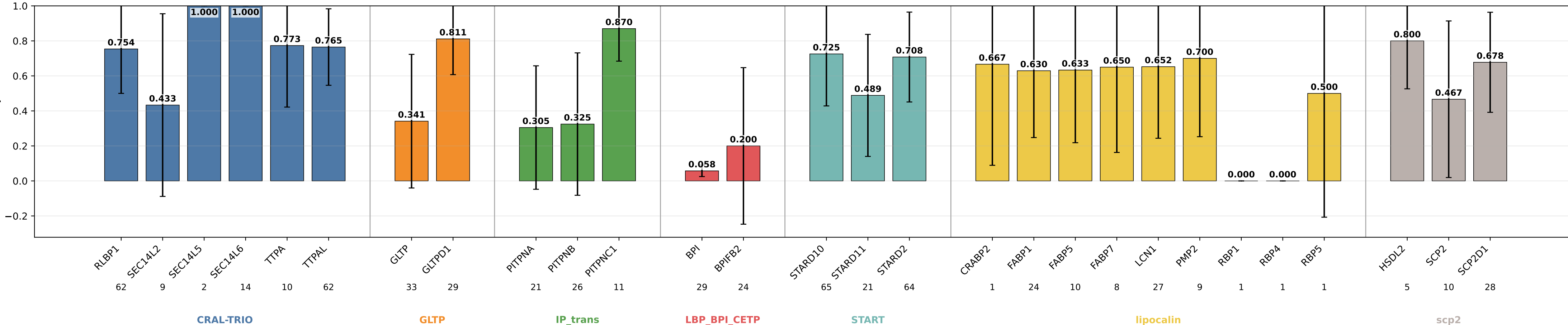
geometric_edge_mlp_protgeom_family_neutral sensitivity by subgroup geometric_edge_mlp_protgeom_family_neutral | class weights | lr=0.0001 | weight_decay=0.01 | final_m=4 | final_dropout=0.1 | hiddim=8 | heads=8 | batch=16 | ep=120 | seeds=0,1,2,3,4
