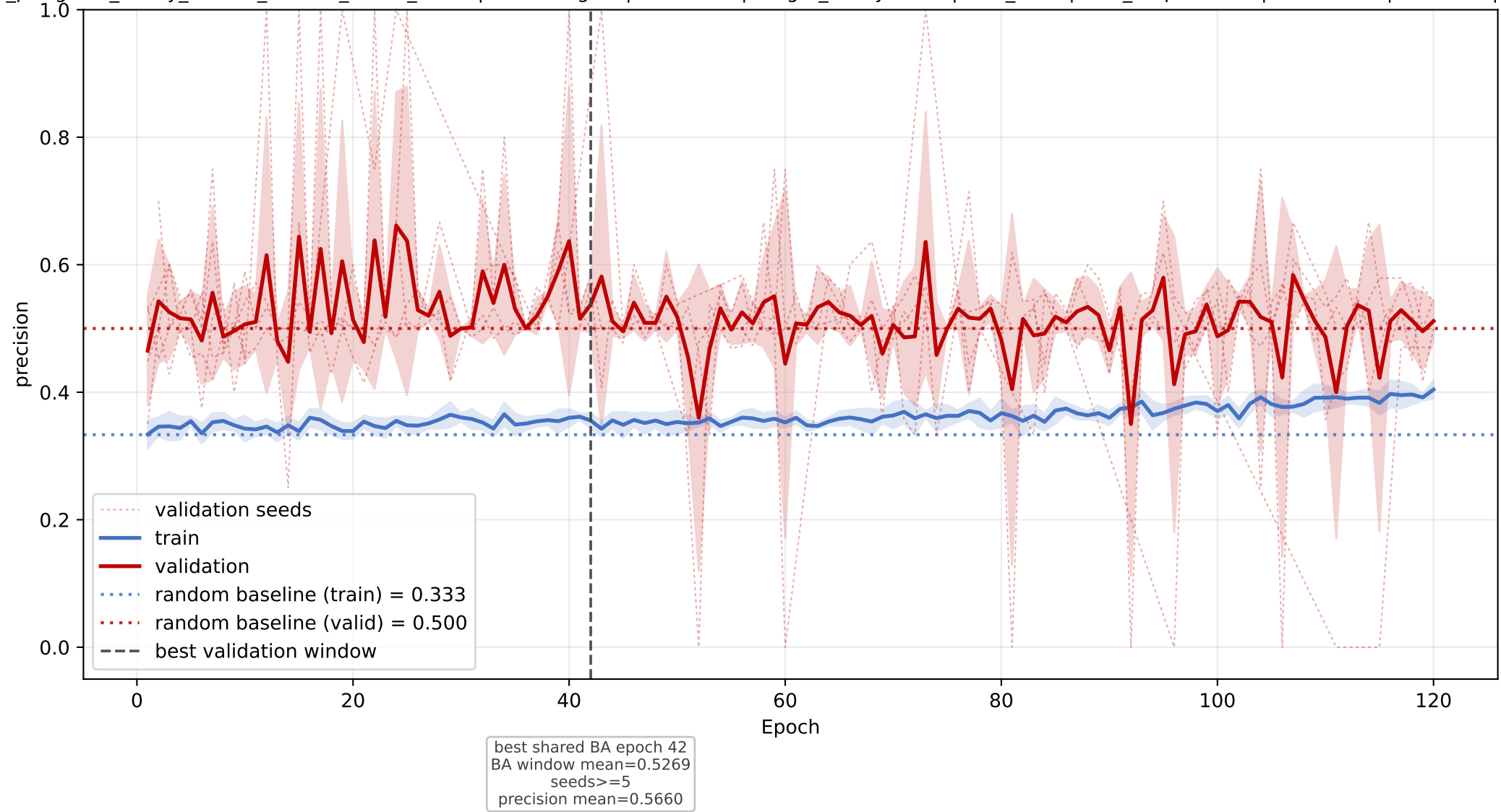
GLTP: mean precision learning curve across seeds
