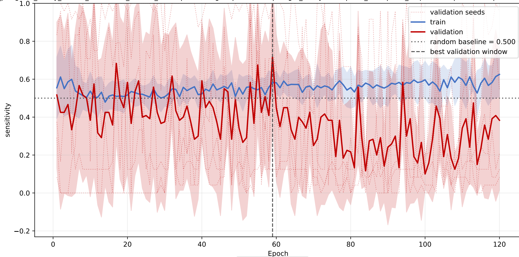
LBP_BPI_CETP: mean sensitivity learning curve across seeds
