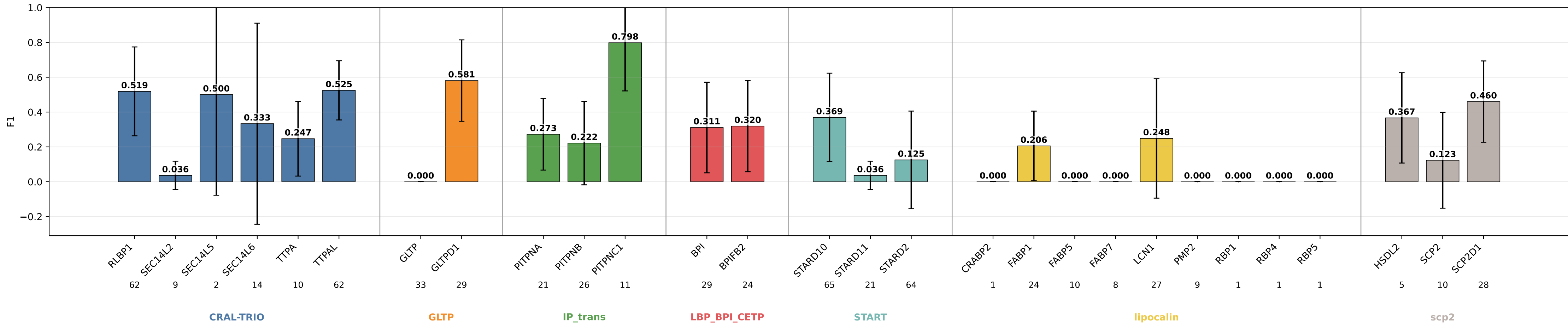
geometric_edge_mlp_protgeom_family_neutral_normalized_bilinear_fusion_bilinear_norm F1 by subgroup geometric_edge_mlp_protgeom_family_neutral_normalized_bilinear_fusion_bilinear_norm | class weights | lr=0.0001 | weight_decay=0.01 | final_m=4 | final_dropout=0.1 | hiddim=8 | heads=8 | batch=16 | ep=120 | seeds=0,1,2,3,4
