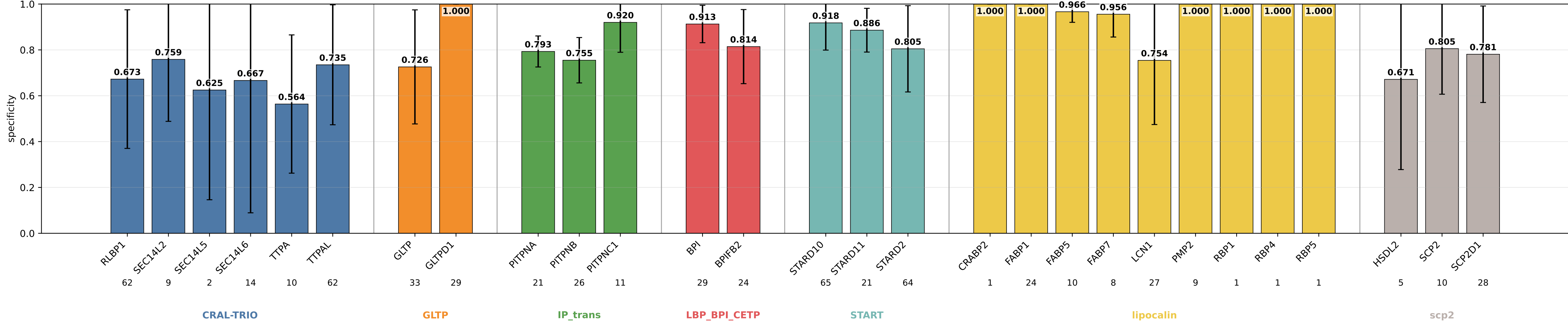
geometric_edge_mlp_protgeom_family_neutral_normalized_bilinear_fusion_bilinear_norm specificity by subgroup geometric_edge_mlp_protgeom_family_neutral_normalized_bilinear_fusion_bilinear_norm | class weights | lr=0.0001 | weight_decay=0.01 | final_m=4 | final_dropout=0.1 | hiddim=8 | heads=8 | batch=16 | ep=120 | seeds=0,1,2,3,4
