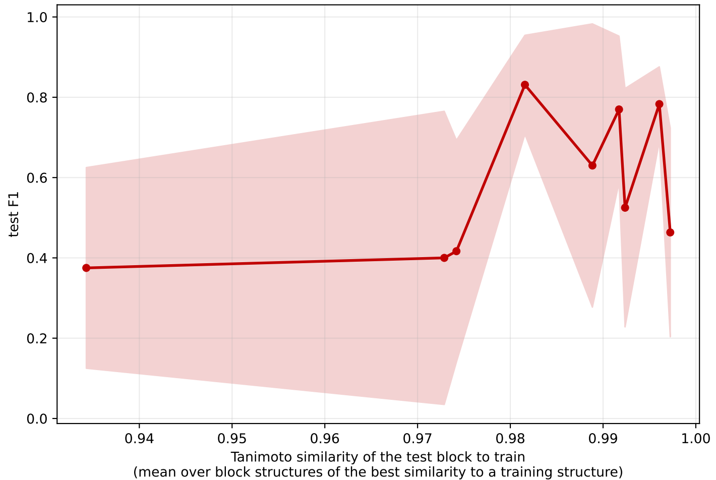
deepclip_f8_normal_mean_ep120 [family_only]
