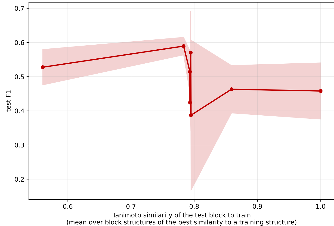
descriptors_head_family_neutral_lipprop [double_coldsplit, random]
