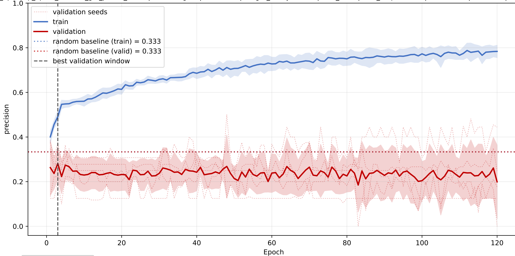
lipocalin: mean precision learning curve across seeds
