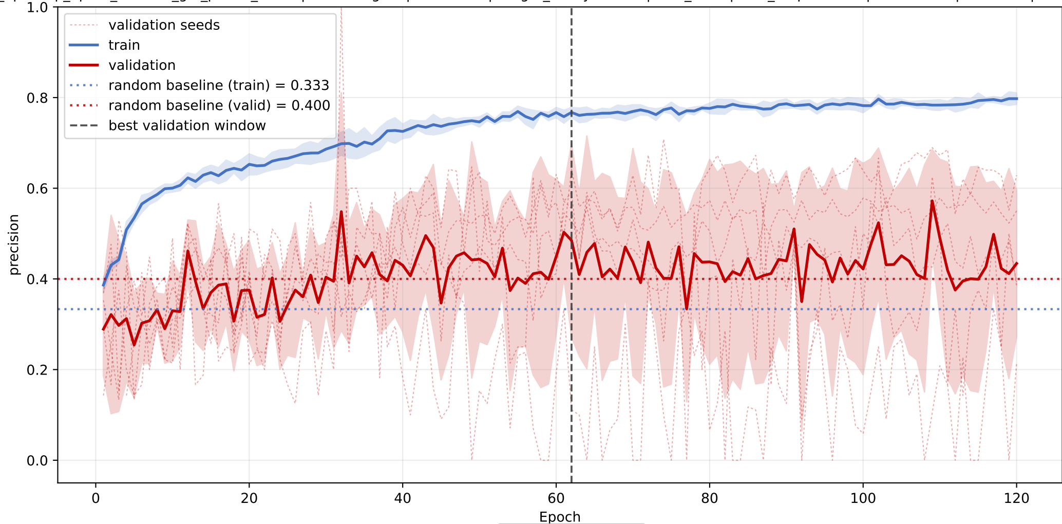
choline: mean precision learning curve across seeds
