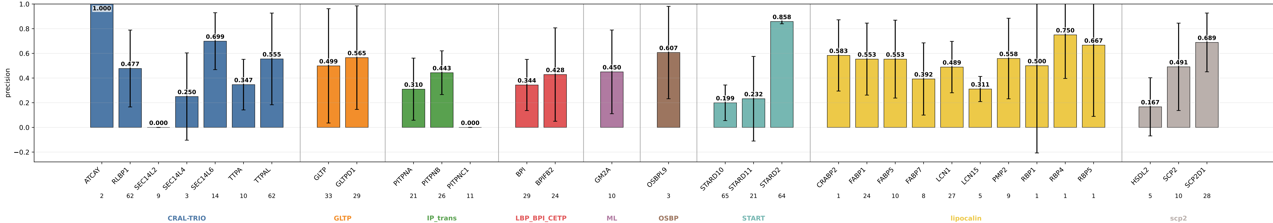
bbp_lcs_rand_fa_nps3mlp_dpt01_wd0001_gm_plm64_hid64 precision by subgroup bbp_lcs_rand_fa_nps3mlp_dpt01_wd0001_gm_plm64_hid64 | class weights | lr=0.0001 | weight_decay=0.001 | final_m=4 | final_dropout=0.1 | hiddim=64 | heads=8 | batch=16 | ep=120 | seeds=0,1,2,3,4
