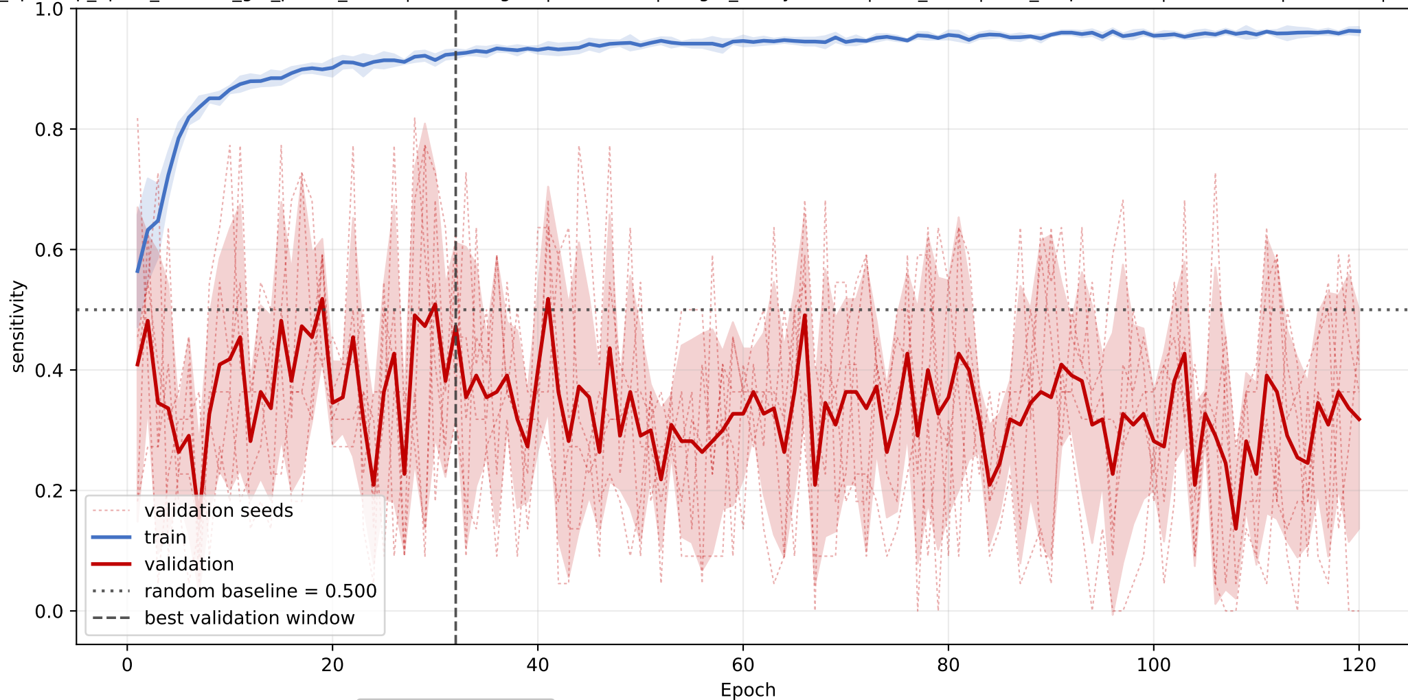
scp2: mean sensitivity learning curve across seeds
