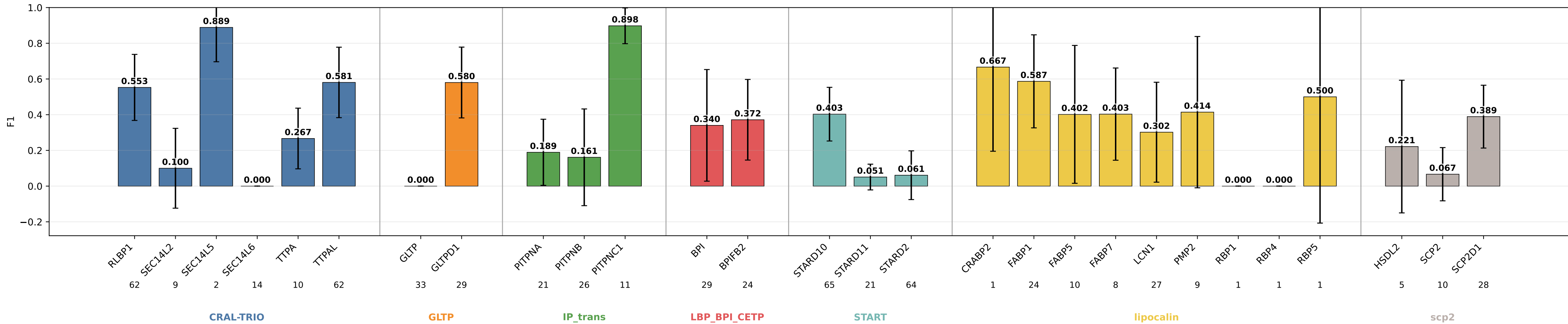
geometric_edge_mlp_protgeom_family_neutral_normalized_bilinear_fusion_bilinear_norm_cross_forced F1 by subgroup geometric_edge_mlp_protgeom_family_neutral_normalized_bilinear_fusion_bilinear_norm_cross_forced | class weights | lr=0.0001 | weight_decay=0.01 | final_m=4 | final_dropout=0.1 | hiddim=8 | heads=8 | batch=16 | ep=120 | seeds=0,1,2,3,4
