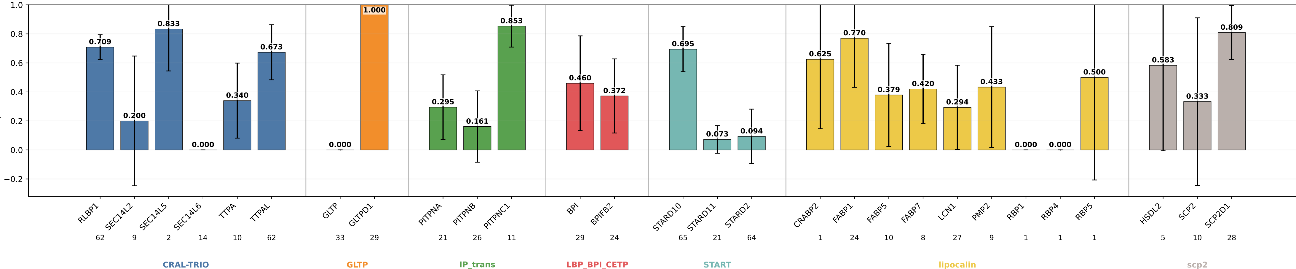
geometric_edge_mlp_protgeom_family_neutral_normalized_bilinear_fusion_bilinear_norm_cross_forced precision by subgroup geometric_edge_mlp_protgeom_family_neutral_normalized_bilinear_fusion_bilinear_norm_cross_forced | class weights | lr=0.0001 | weight_decay=0.01 | final_m=4 | final_dropout=0.1 | hiddim=8 | heads=8 | batch=16 | ep=120 | seeds=0,1,2,3,4
