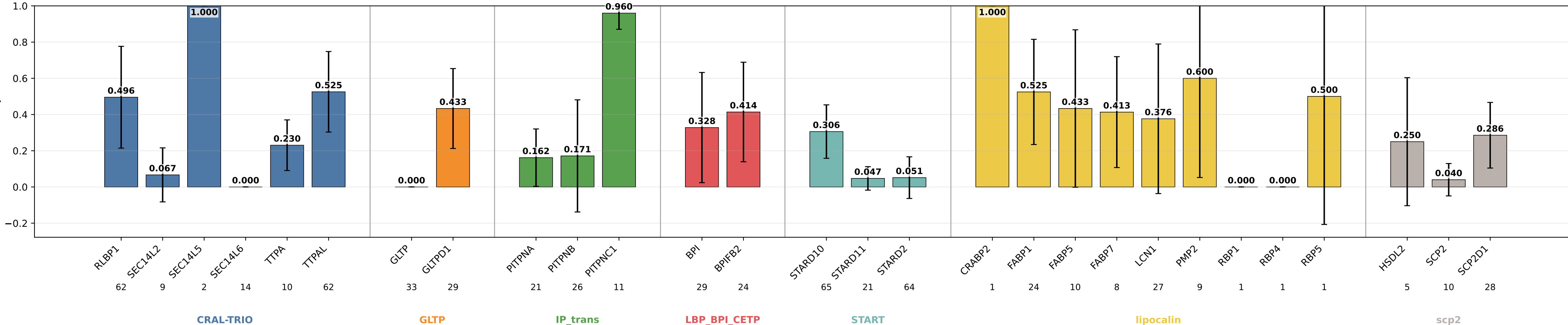
geometric_edge_mlp_protgeom_family_neutral_normalized_bilinear_fusion_bilinear_norm_cross_forced sensitivity by subgroup geometric_edge_mlp_protgeom_family_neutral_normalized_bilinear_fusion_bilinear_norm_cross_forced | class weights | lr=0.0001 | weight_decay=0.01 | final_m=4 | final_dropout=0.1 | hiddim=8 | heads=8 | batch=16 | ep=120 | seeds=0,1,2,3,4
