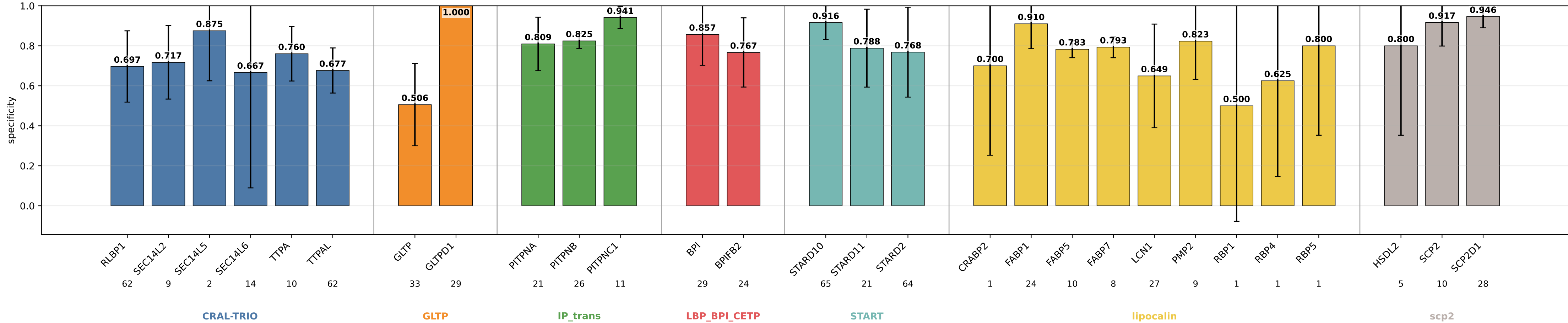
geometric_edge_mlp_protgeom_family_neutral_normalized_bilinear_fusion_bilinear_norm_cross_forced specificity by subgroup geometric_edge_mlp_protgeom_family_neutral_normalized_bilinear_fusion_bilinear_norm_cross_forced | class weights | lr=0.0001 | weight_decay=0.01 | final_m=4 | final_dropout=0.1 | hiddim=8 | heads=8 | batch=16 | ep=120 | seeds=0,1,2,3,4
