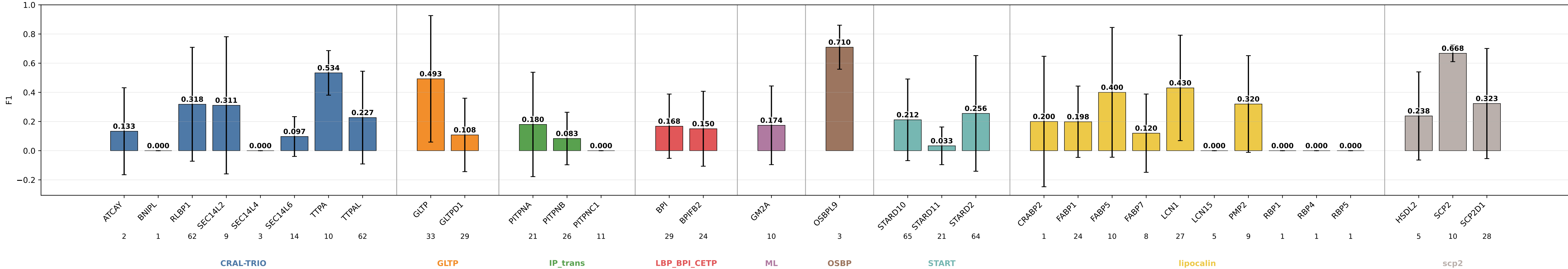
geometric_edge_mlp_protgeom_family_neutral_normalized_bilinear_fusion_bilinear_norm_lcs_esm3_hid64 F1 by subgroup geometric_edge_mlp_protgeom_family_neutral_normalized_bilinear_fusion_bilinear_norm_lcs_esm3_hid64 | class weights | lr=0.0001 | weight_decay=0.01 | final_m=4 | final_dropout=0.1 | hiddim=64 | heads=8 | batch=16 | ep=120 | seeds=0,1,2,3,4
