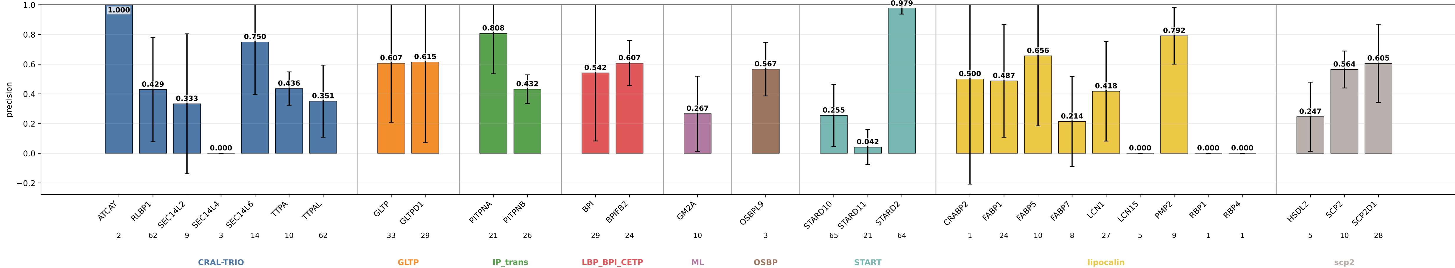
geometric_edge_mlp_protgeom_family_neutral_normalized_bilinear_fusion_bilinear_norm_lcs_esm3_hid64 precision by subgroup geometric_edge_mlp_protgeom_family_neutral_normalized_bilinear_fusion_bilinear_norm_lcs_esm3_hid64 | class weights | lr=0.0001 | weight_decay=0.01 | final_m=4 | final_dropout=0.1 | hiddim=64 | heads=8 | batch=16 | ep=120 | seeds=0,1,2,3,4
