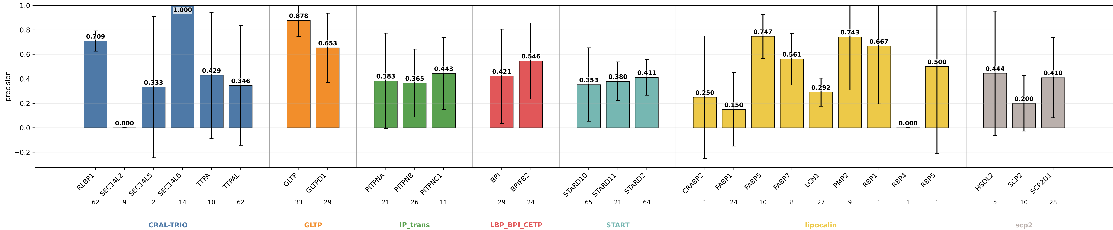
thematical_paths_geom_chem_orthogonal_init_hid16 precision by subgroup thematical_paths_geom_chem_orthogonal_init_hid16 | class weights | lr=0.0001 | weight_decay=0.01 | final_m=4 | final_dropout=0.1 | hiddim=16 | heads=8 | batch=16 | ep=120 | seeds=0,1,2,3,4
