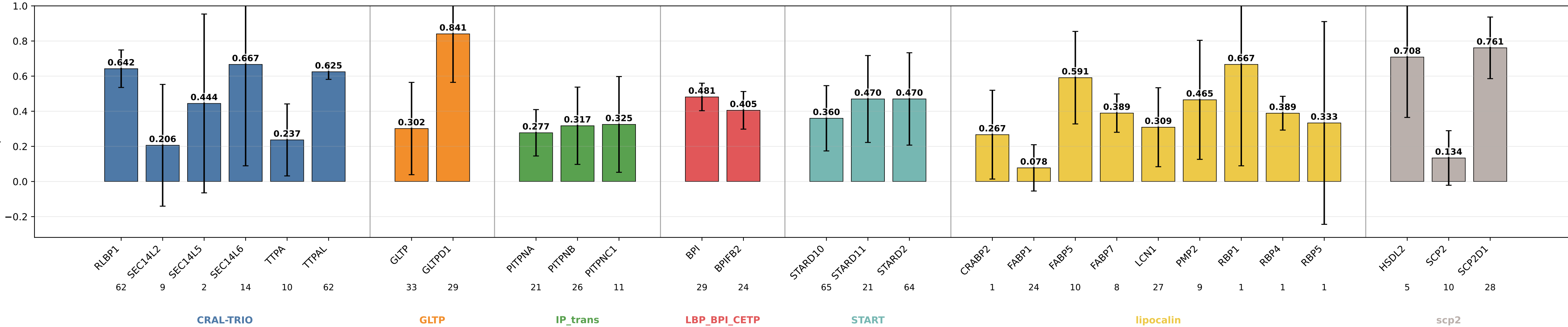
thematical_paths_geom_chem_orthogonal_init_no_volume precision by subgroup thematical_paths_geom_chem_orthogonal_init_no_volume | class weights | lr=0.0001 | weight_decay=0.01 | final_m=4 | final_dropout=0.1 | hiddim=8 | heads=8 | batch=16 | ep=120 | seeds=0,1,2,3,4
