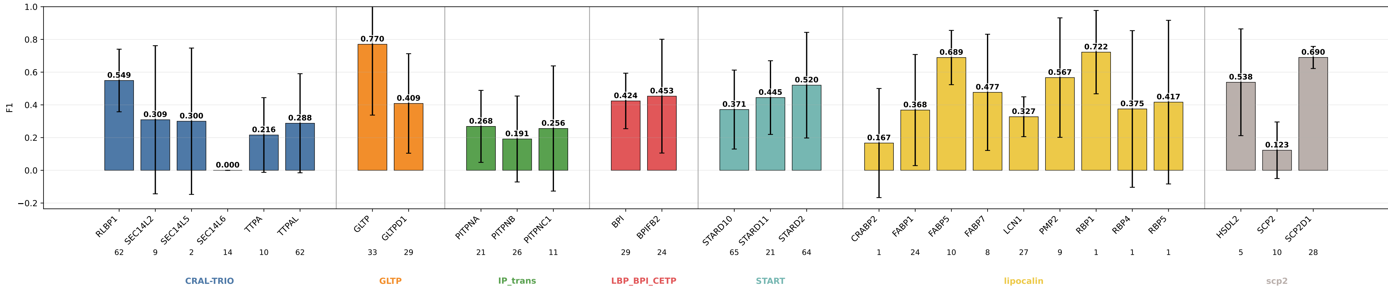
thematical_paths_geom_chem_orthogonal_init_pair_priors F1 by subgroup thematical_paths_geom_chem_orthogonal_init_pair_priors | class weights | lr=0.0001 | weight_decay=0.01 | final_m=4 | final_dropout=0.1 | hiddim=8 | heads=8 | batch=16 | ep=120 | seeds=0,1,2,3,4
