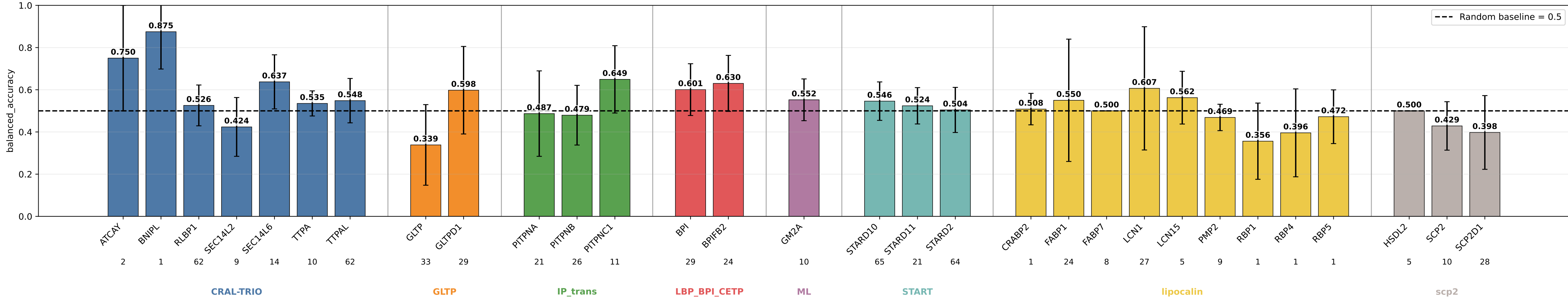
geometric_edge_mlp_protgeom_family_neutral_normalized_bilinear_fusion_bilinear_norm_lcs_esm3_balanced_lipid_classes_rankprot_advprot | balanced_accuracy by subgroup geometric_edge_mlp_protgeom_family_neutral_normalized_bilinear_fusion_bilinear_norm_lcs_esm3_balanced_lipid_classes_rankprot_advprot | class weights | lr=0.0001 | weight_decay=0.01 | final_m=4 | final_dropout=0.1 | hiddim=8 | heads=8 | batch=64 | ep=120 | seeds=0,1,2,3,4
