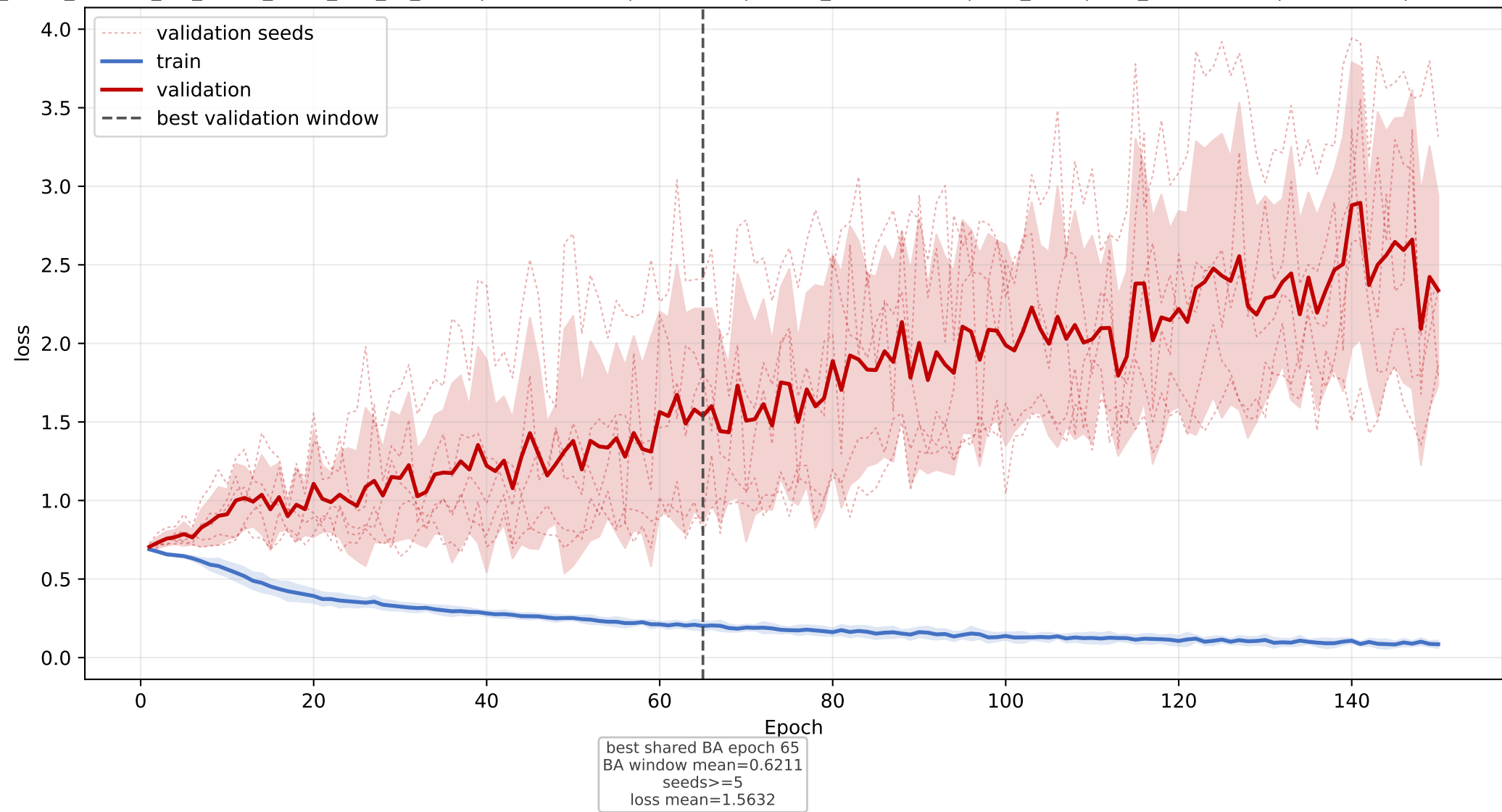
lipocalin: mean loss learning curve across seeds
