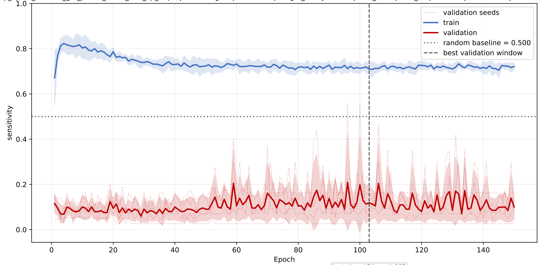
GLTP: mean sensitivity learning curve across seeds
