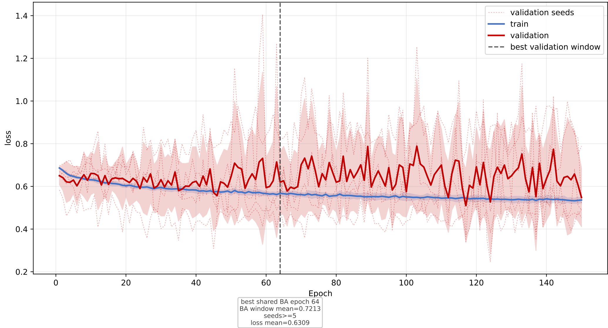
OSBP: mean loss learning curve across seeds
