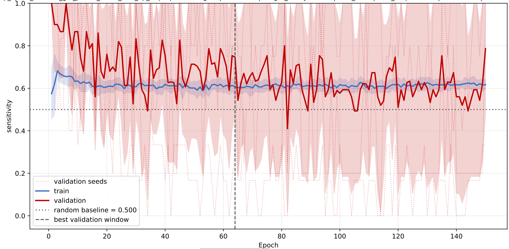
OSBP: mean sensitivity learning curve across seeds
